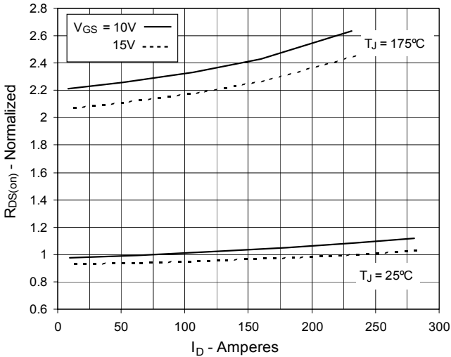
Fig. 5. R_{DS(on)} Normalized to I_D = 80\text{A} Value vs. Drain Current
